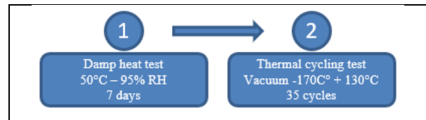
Figure 1 - Schematic principle of cumulative ageing tests
